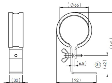
fixing clamp
